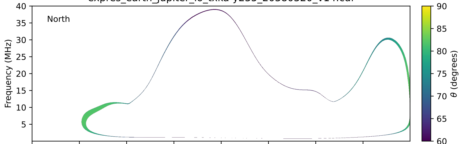
expres_earth_jupiter_io_txka-y235_20380320_v14.cdf
