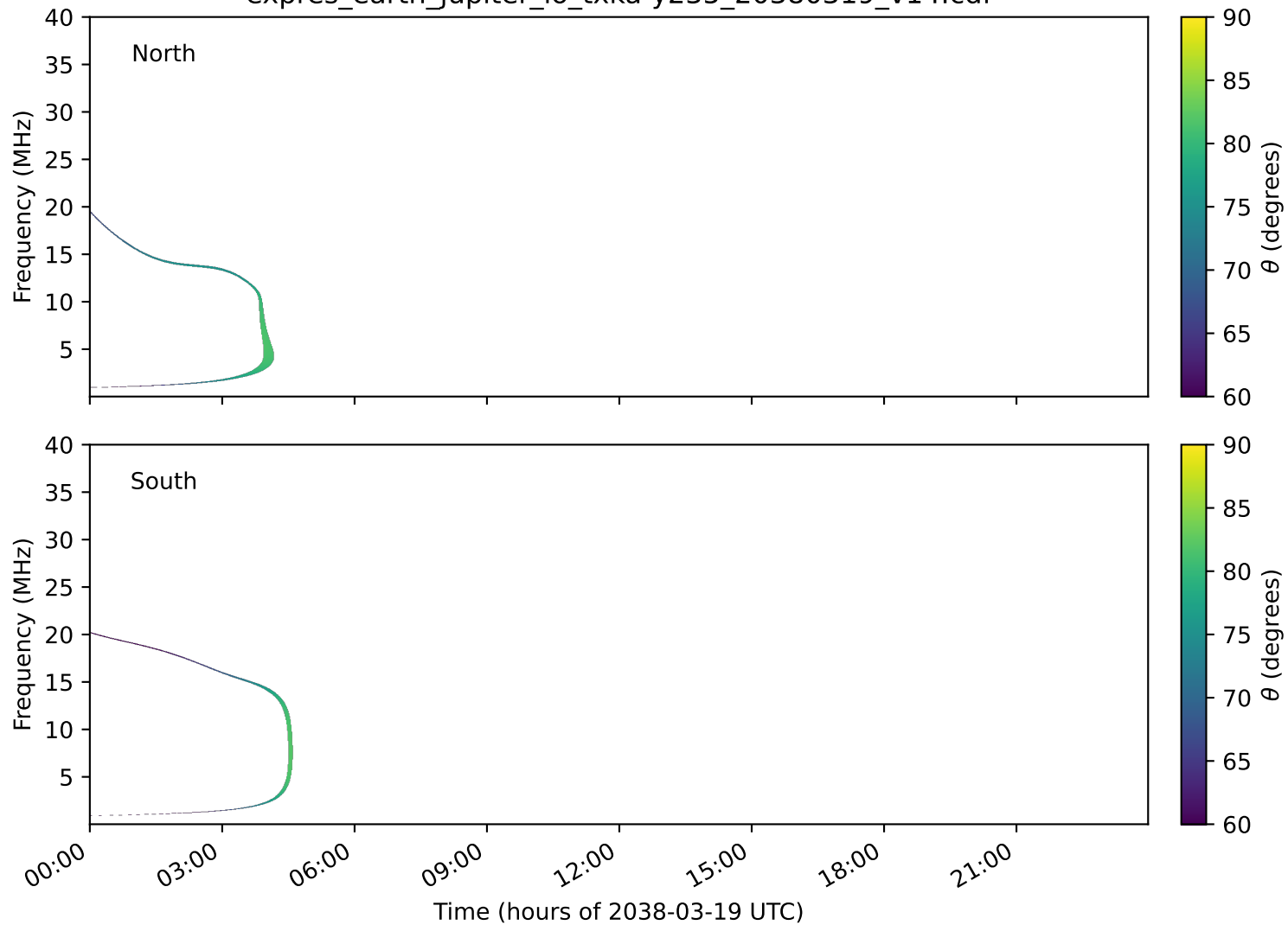
expres_earth_jupiter_io_txka-y235_20380319_v14.cdf
