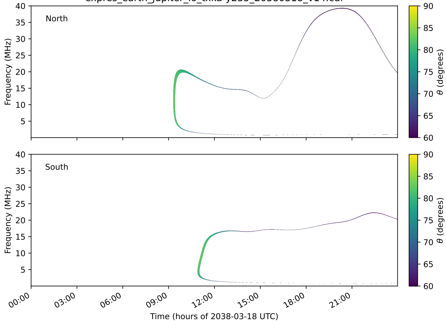
expres_earth_jupiter_io_txka-y235_20380318_v14.cdf
