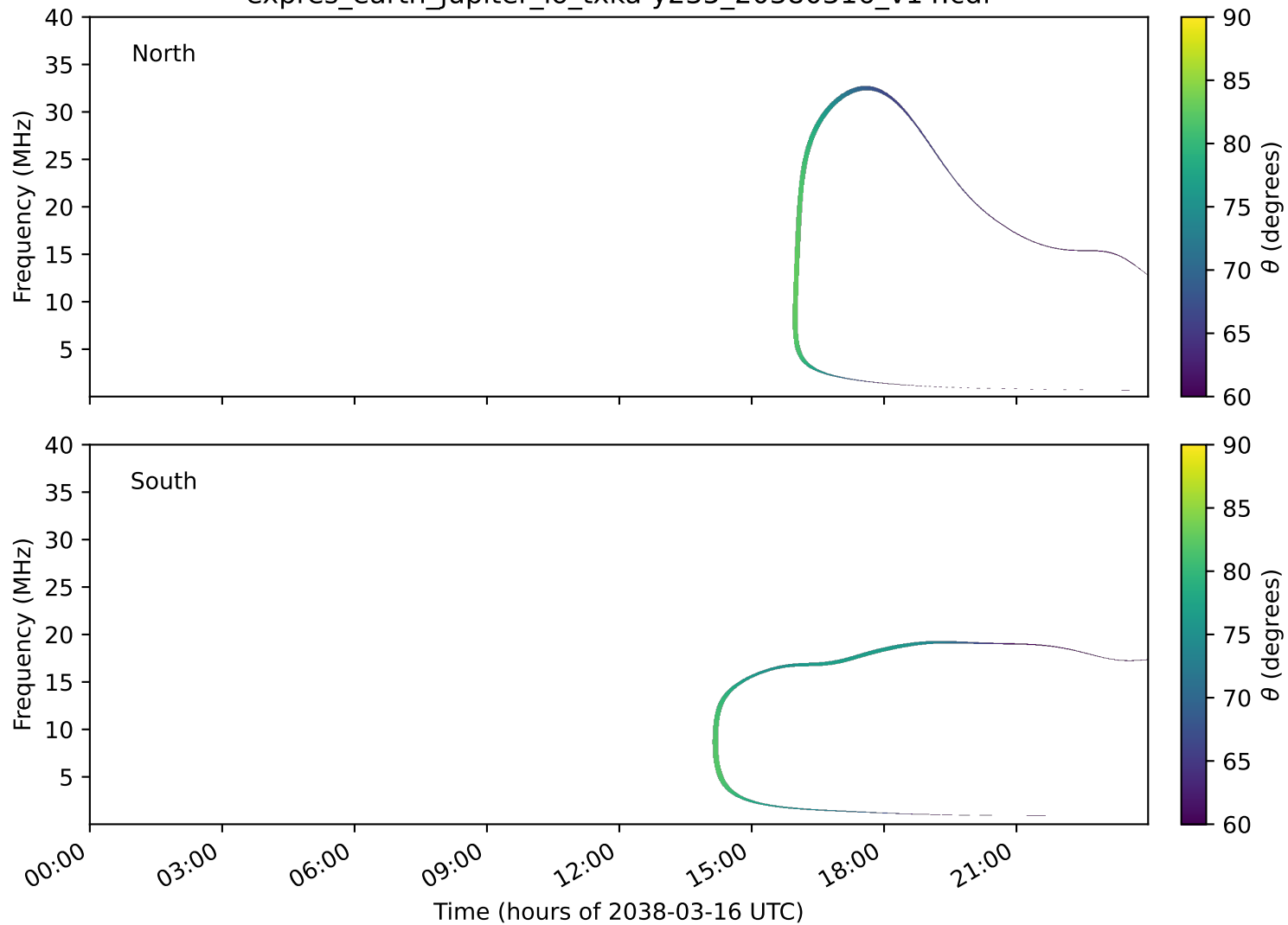
expres_earth_jupiter_io_txka-y235_20380316_v14.cdf
