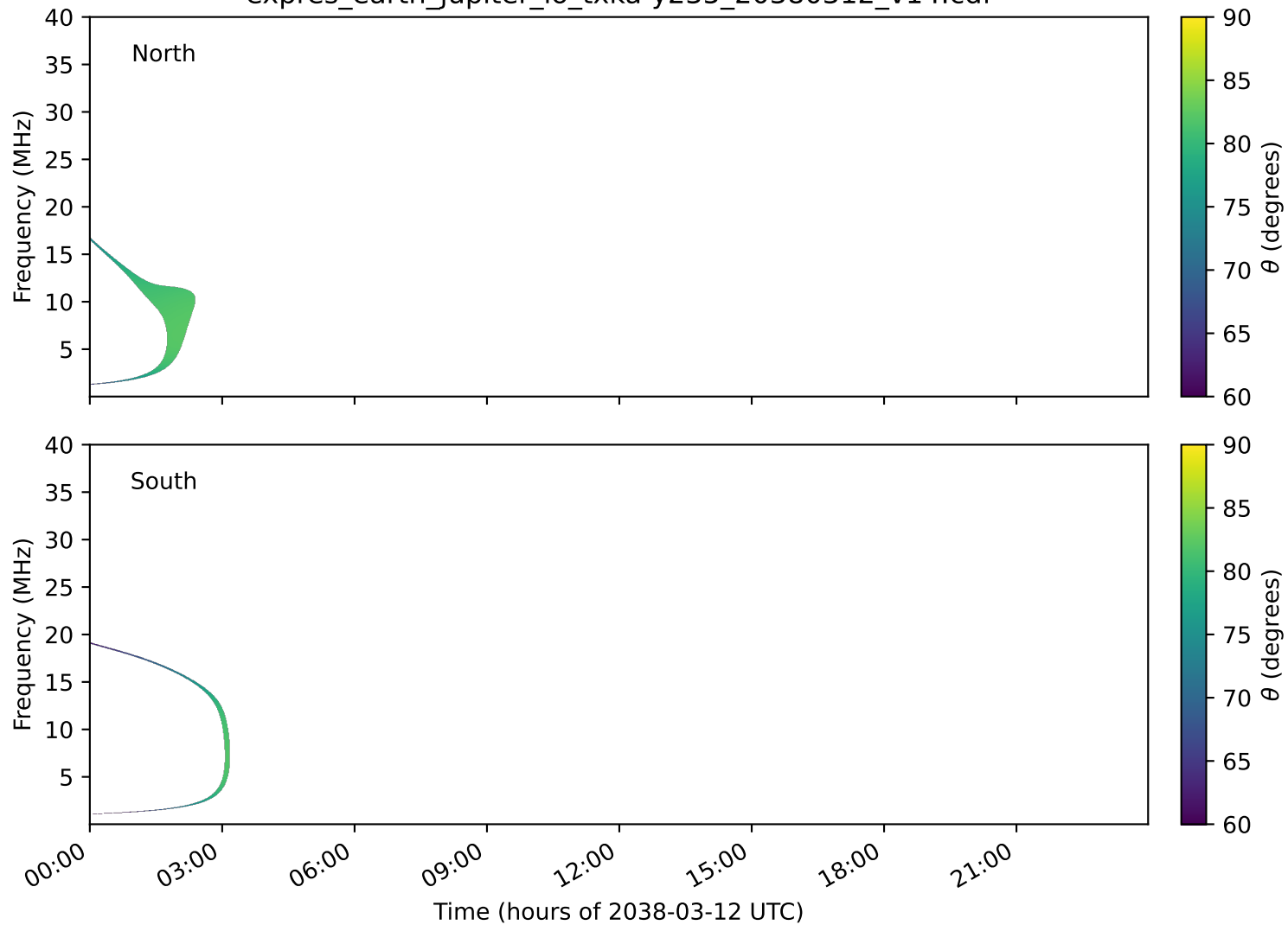
expres_earth_jupiter_io_txka-y235_20380312_v14.cdf
