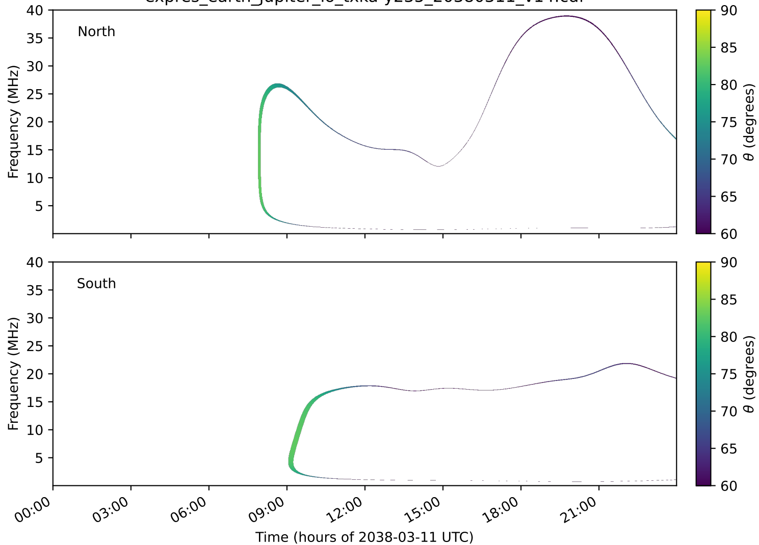
expres_earth_jupiter_io_txka-y235_20380311_v14.cdf
