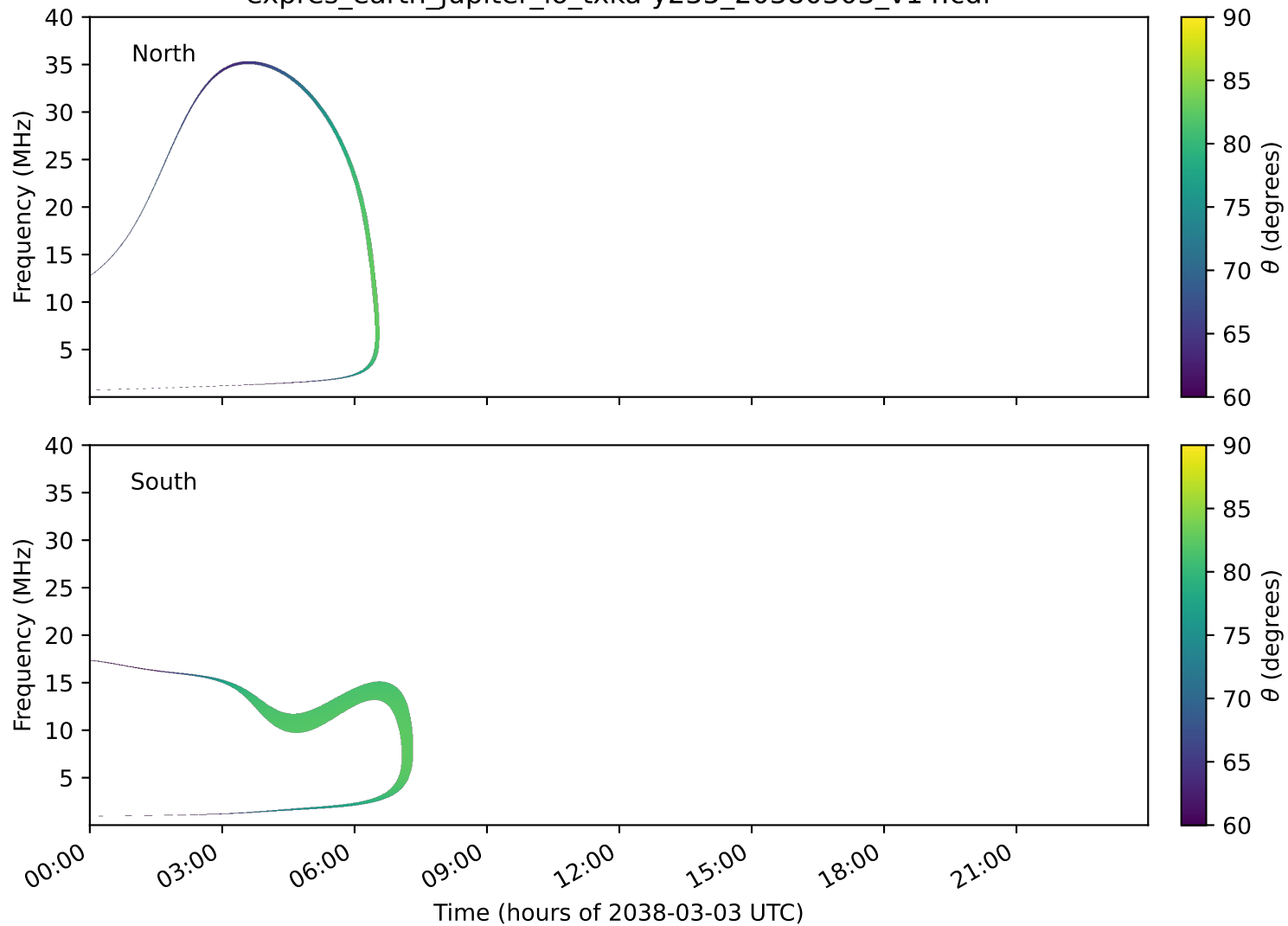
expres_earth_jupiter_io_txka-y235_20380303_v14.cdf
