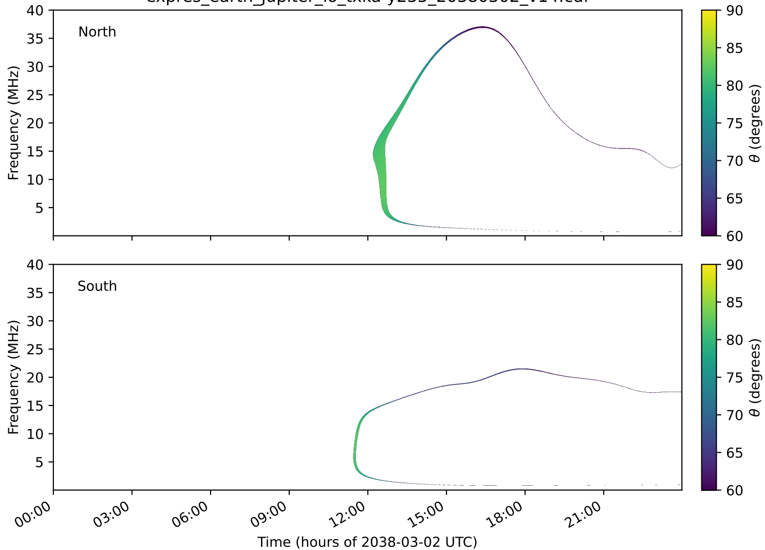
expres_earth_jupiter_io_txka-y235_20380302_v14.cdf
