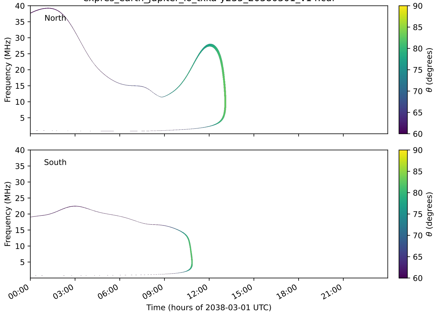
expres_earth_jupiter_io_txka-y235_20380301_v14.cdf
