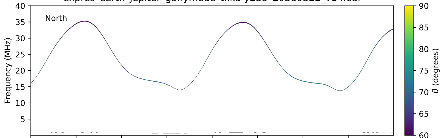
expres_earth_jupiter_ganymede_txka-y235_20380322_v14.cdf
