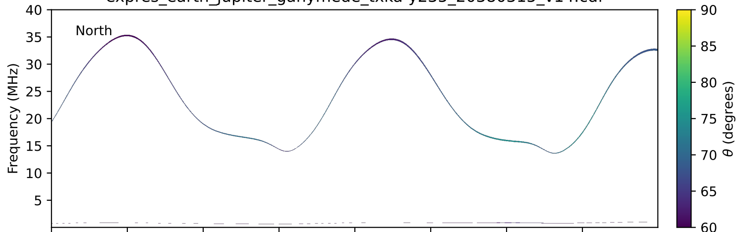
expres_earth_jupiter_ganymede_txka-y235_20380315_v14.cdf
