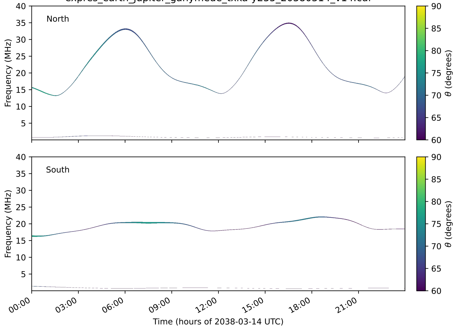
expres_earth_jupiter_ganymede_txka-y235_20380314_v14.cdf
