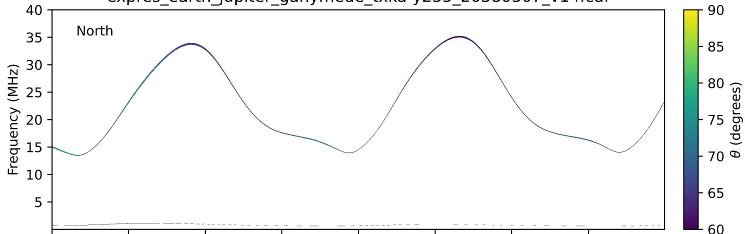
expres_earth_jupiter_ganymede_txka-y235_20380307_v14.cdf
