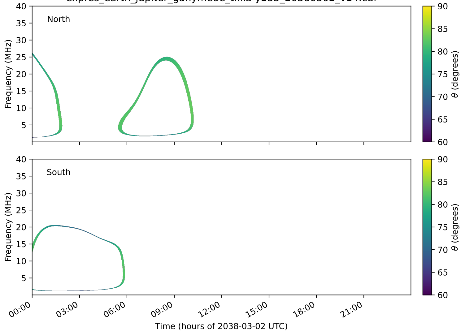
expres_earth_jupiter_ganymede_txka-y235_20380302_v14.cdf
