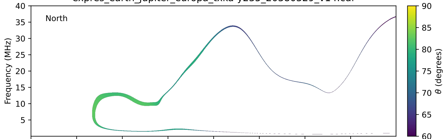
expres_earth_jupiter_europa_txka-y235_20380329_v14.cdf
