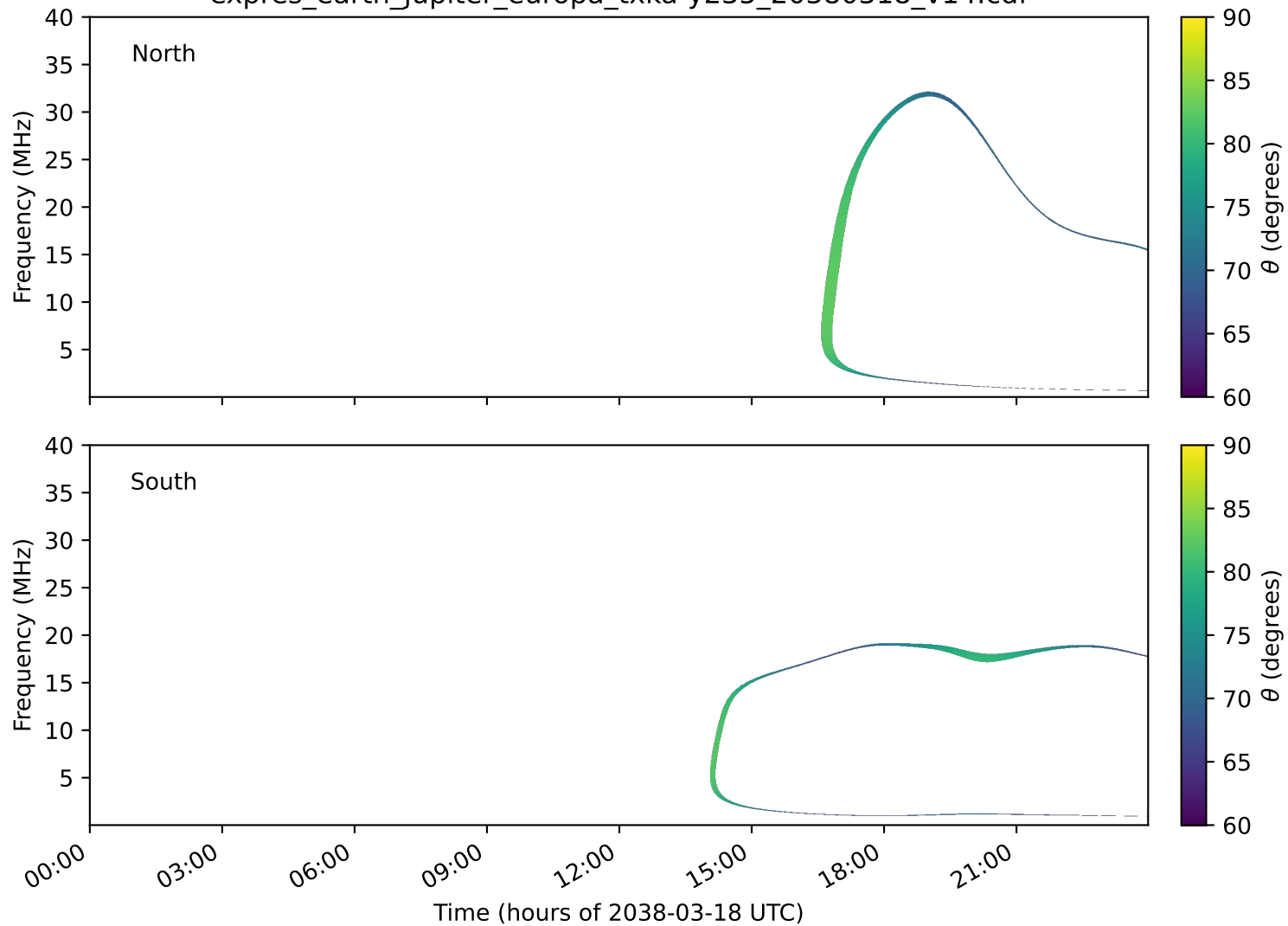
expres_earth_jupiter_europa_txka-y235_20380318_v14.cdf
