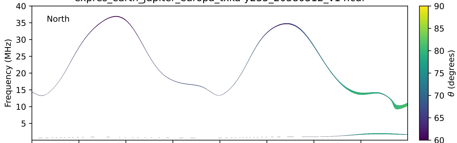
expres_earth_jupiter_europa_txka-y235_20380312_v14.cdf
