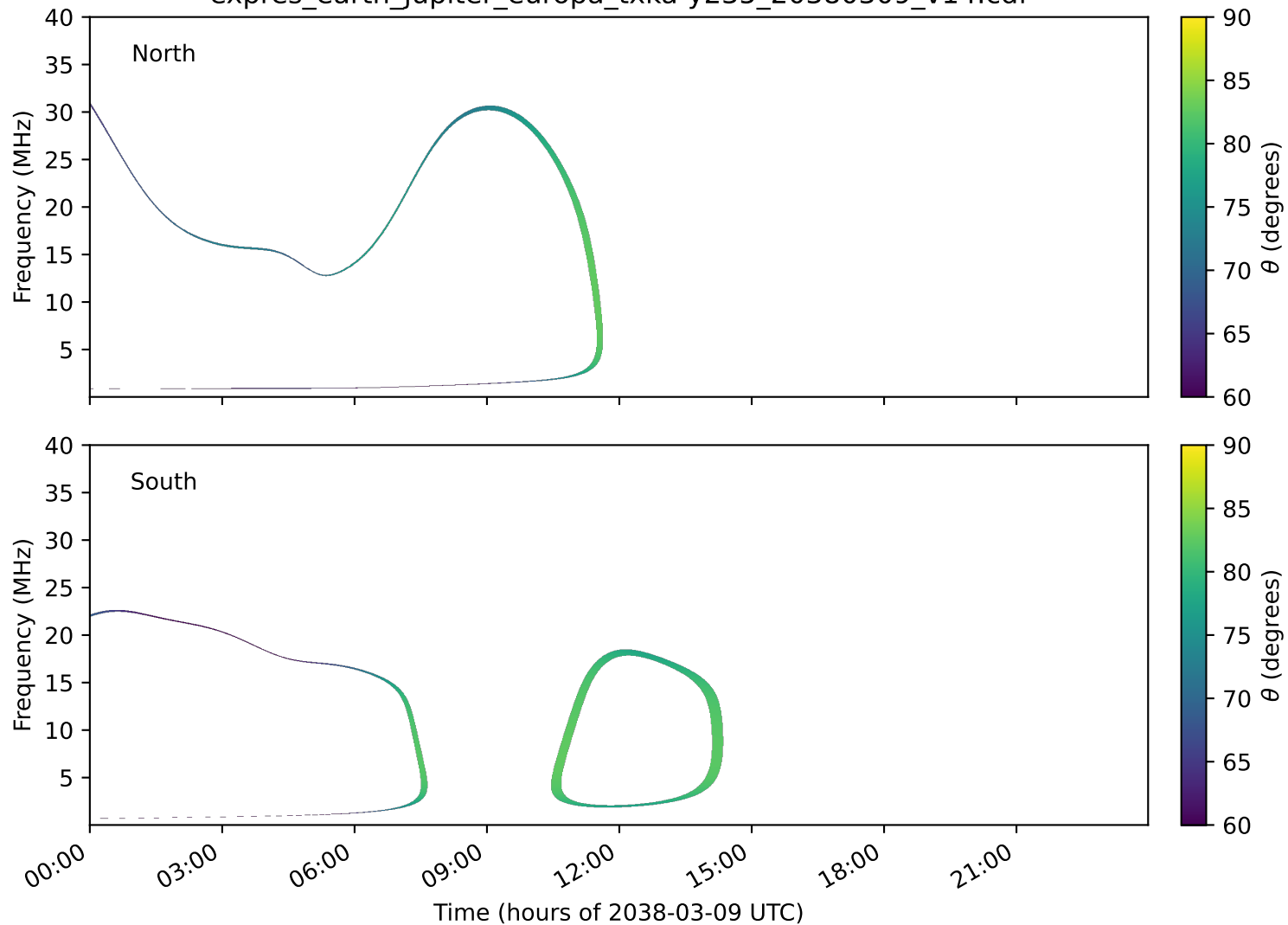
expres_earth_jupiter_europa_txka-y235_20380309_v14.cdf
