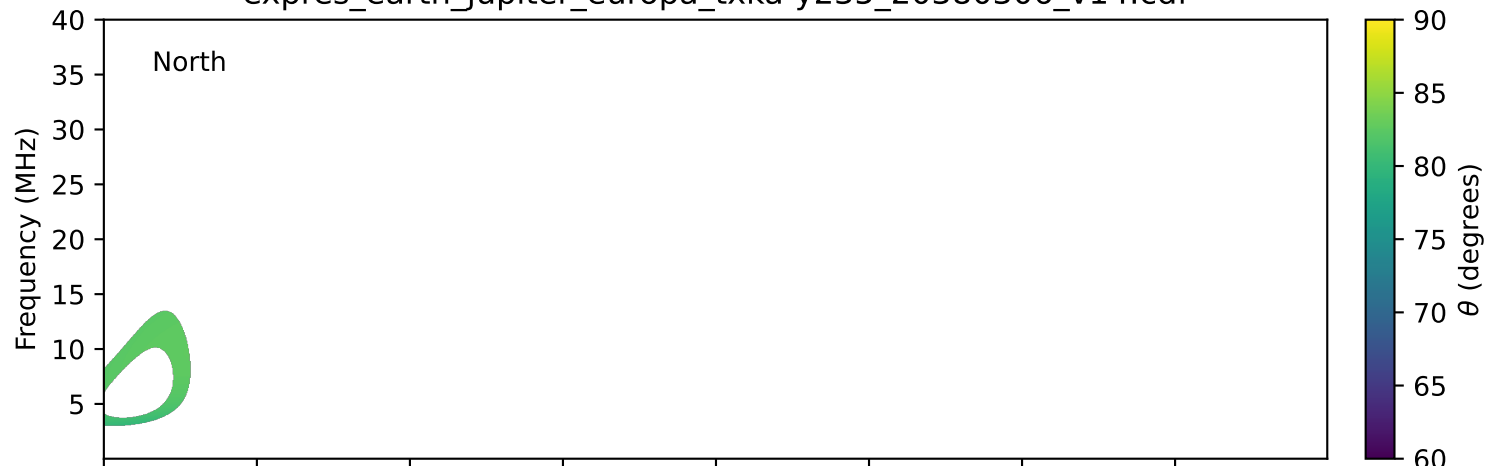
expres_earth_jupiter_europa_txka-y235_20380306_v14.cdf
