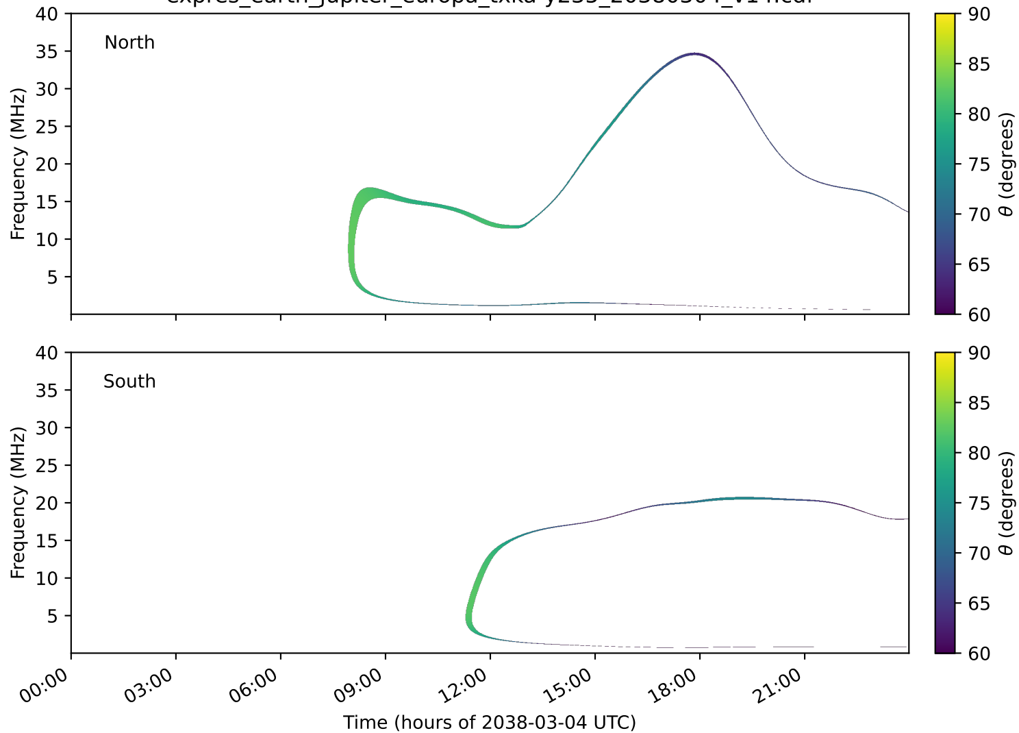
expres_earth_jupiter_europa_txka-y235_20380304_v14.cdf
