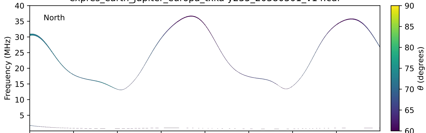
expres_earth_jupiter_europa_txka-y235_20380301_v14.cdf
