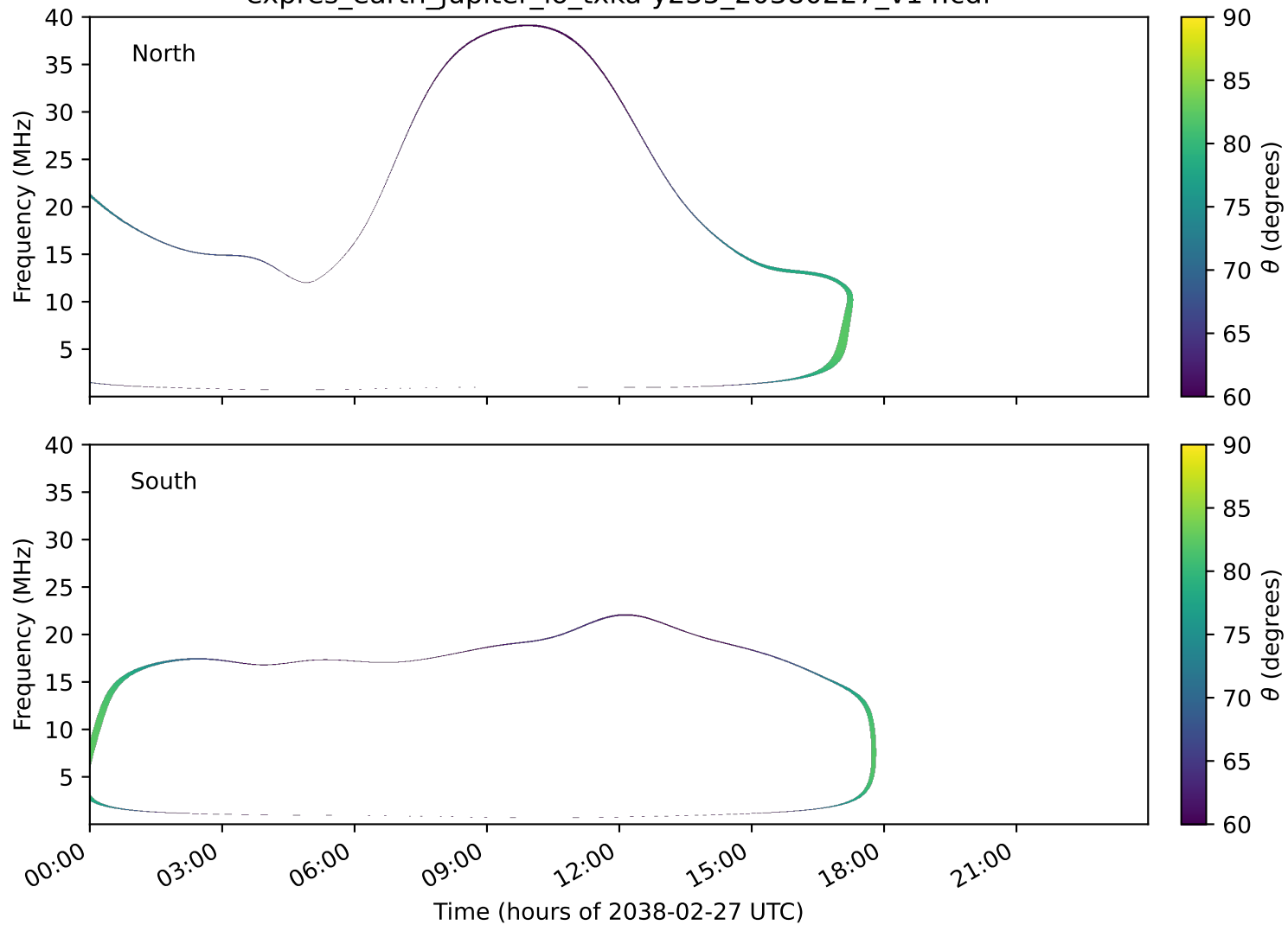
expres_earth_jupiter_io_txka-y235_20380227_v14.cdf
