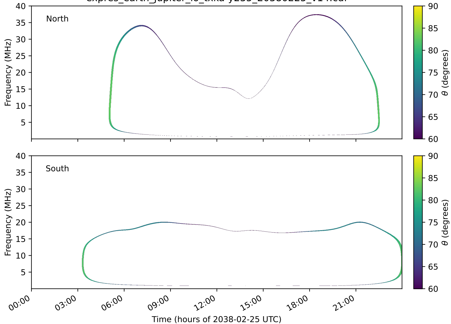
expres_earth_jupiter_io_txka-y235_20380225_v14.cdf
