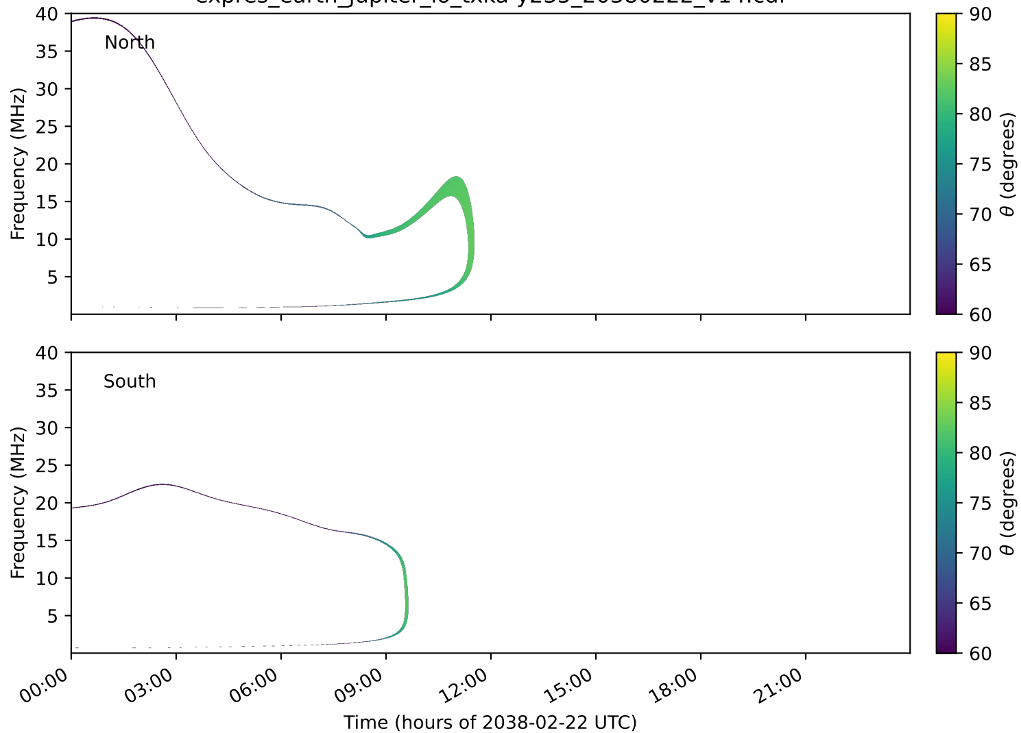
expres_earth_jupiter_io_txka-y235_20380222_v14.cdf
