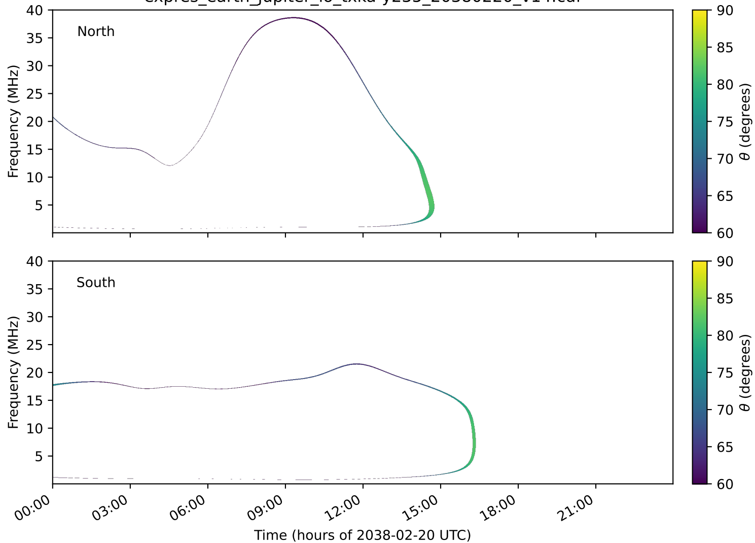
expres_earth_jupiter_io_txka-y235_20380220_v14.cdf
