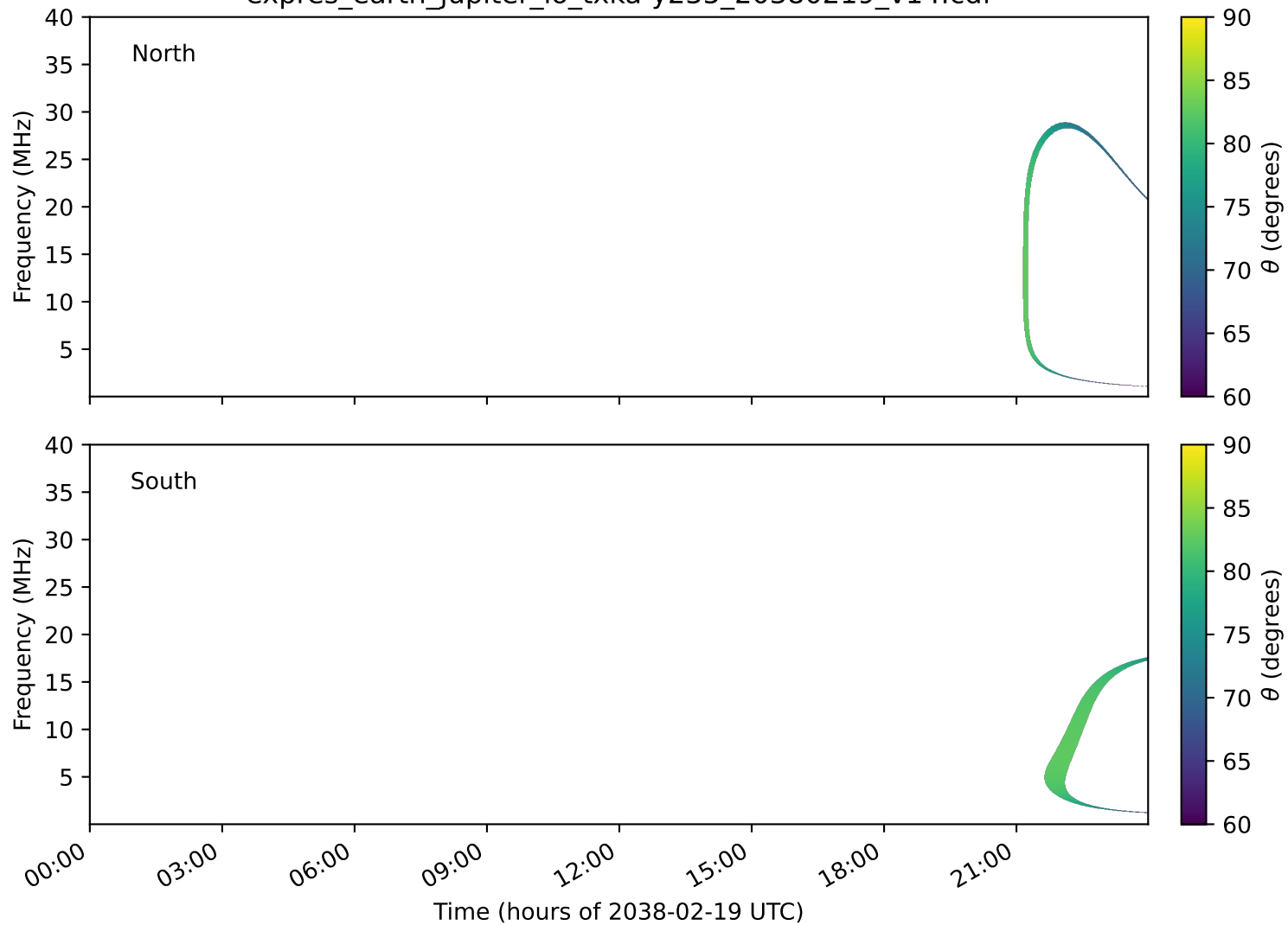
expres_earth_jupiter_io_txka-y235_20380219_v14.cdf
