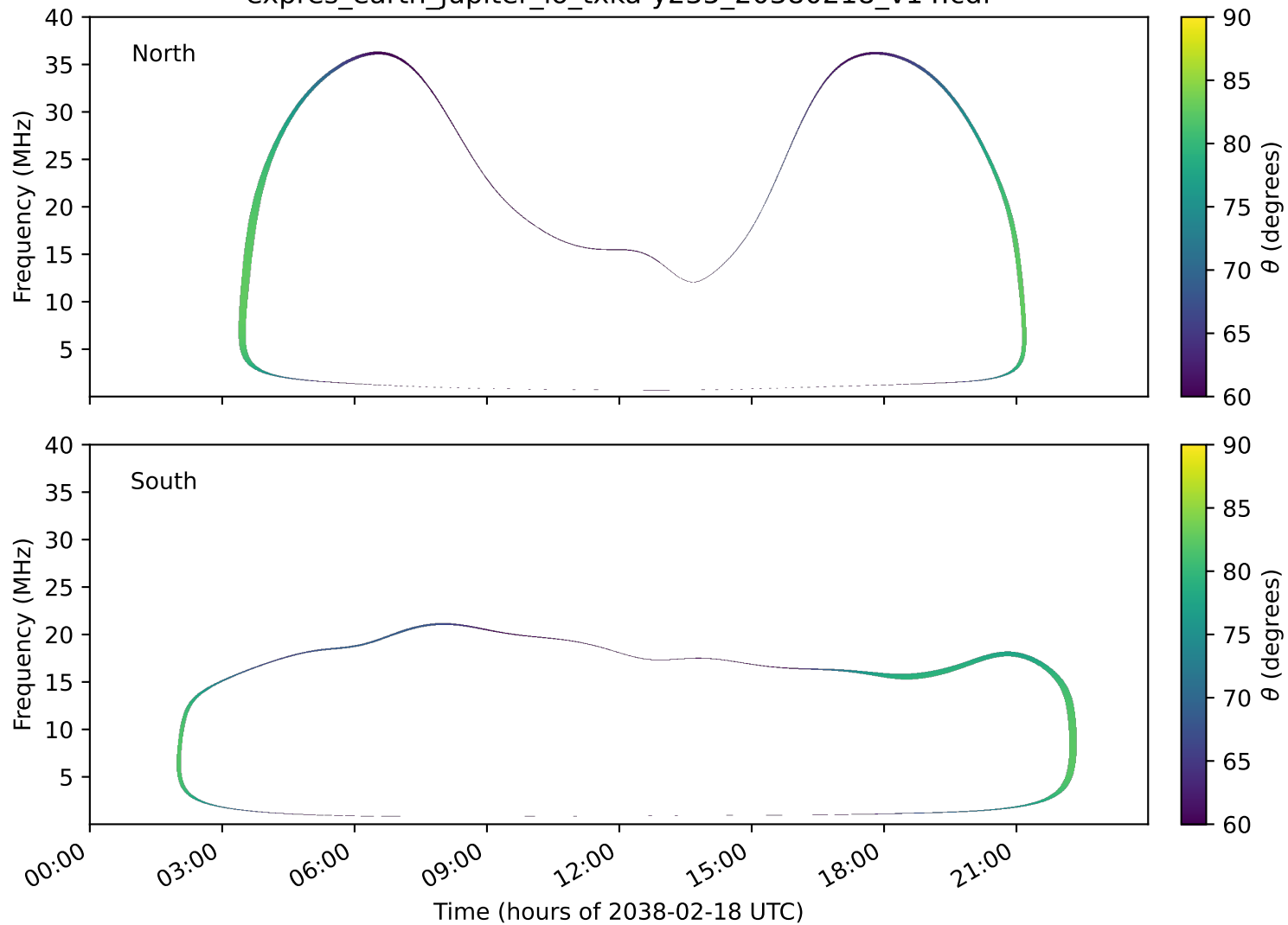
expres_earth_jupiter_io_txka-y235_20380218_v14.cdf
