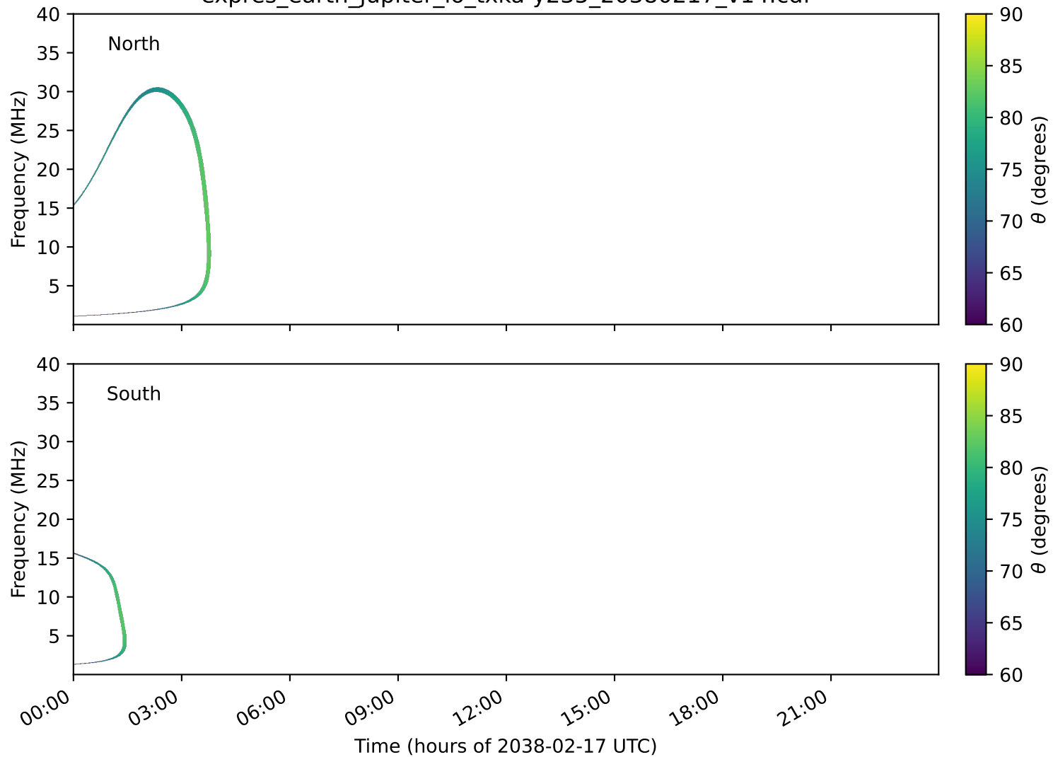
expres_earth_jupiter_io_txka-y235_20380217_v14.cdf
