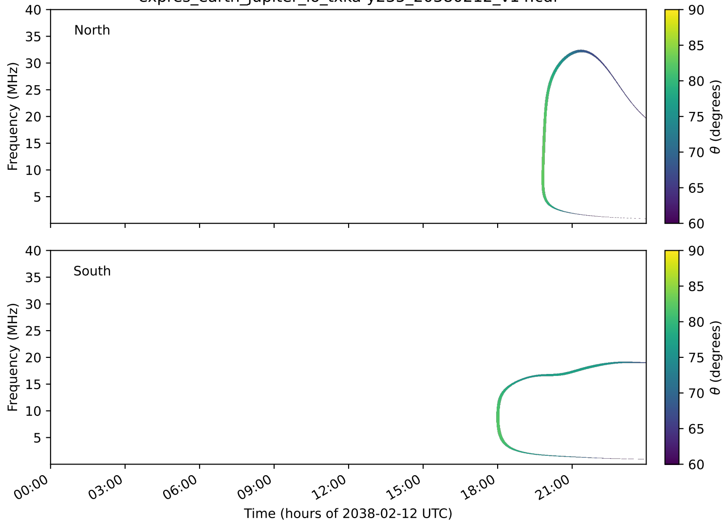
expres_earth_jupiter_io_txka-y235_20380212_v14.cdf
