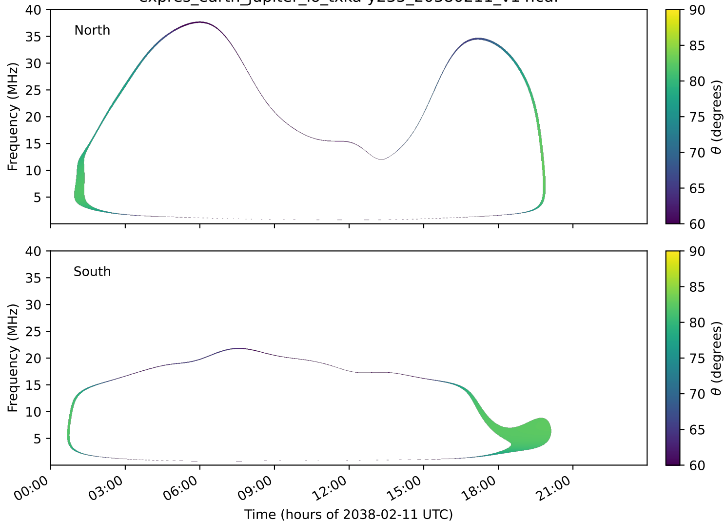
expres_earth_jupiter_io_txka-y235_20380211_v14.cdf
