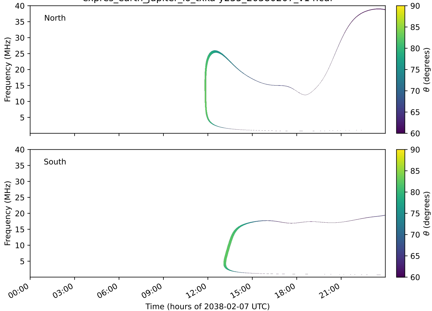
expres_earth_jupiter_io_txka-y235_20380207_v14.cdf
