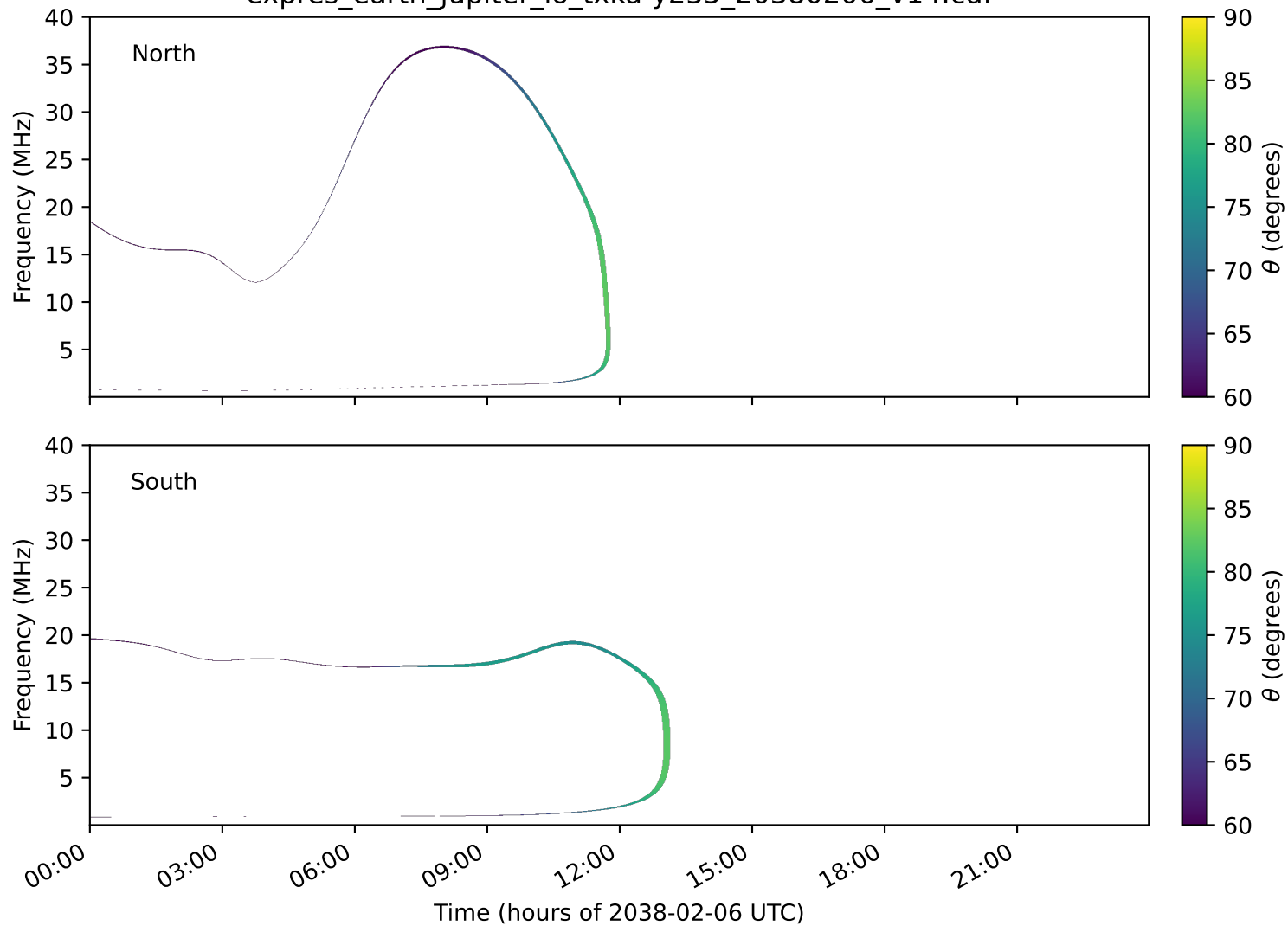
expres_earth_jupiter_io_txka-y235_20380206_v14.cdf
