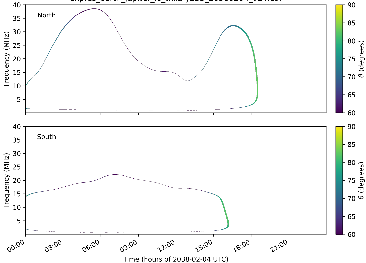
expres_earth_jupiter_io_txka-y235_20380204_v14.cdf
