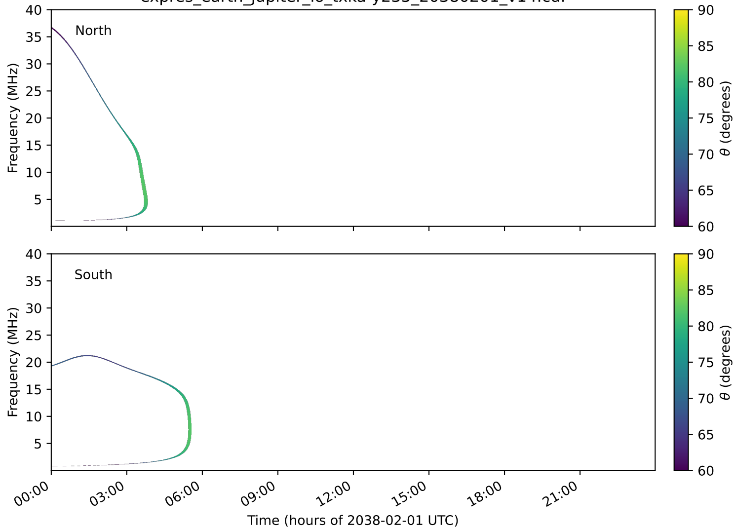
expres_earth_jupiter_io_txka-y235_20380201_v14.cdf
