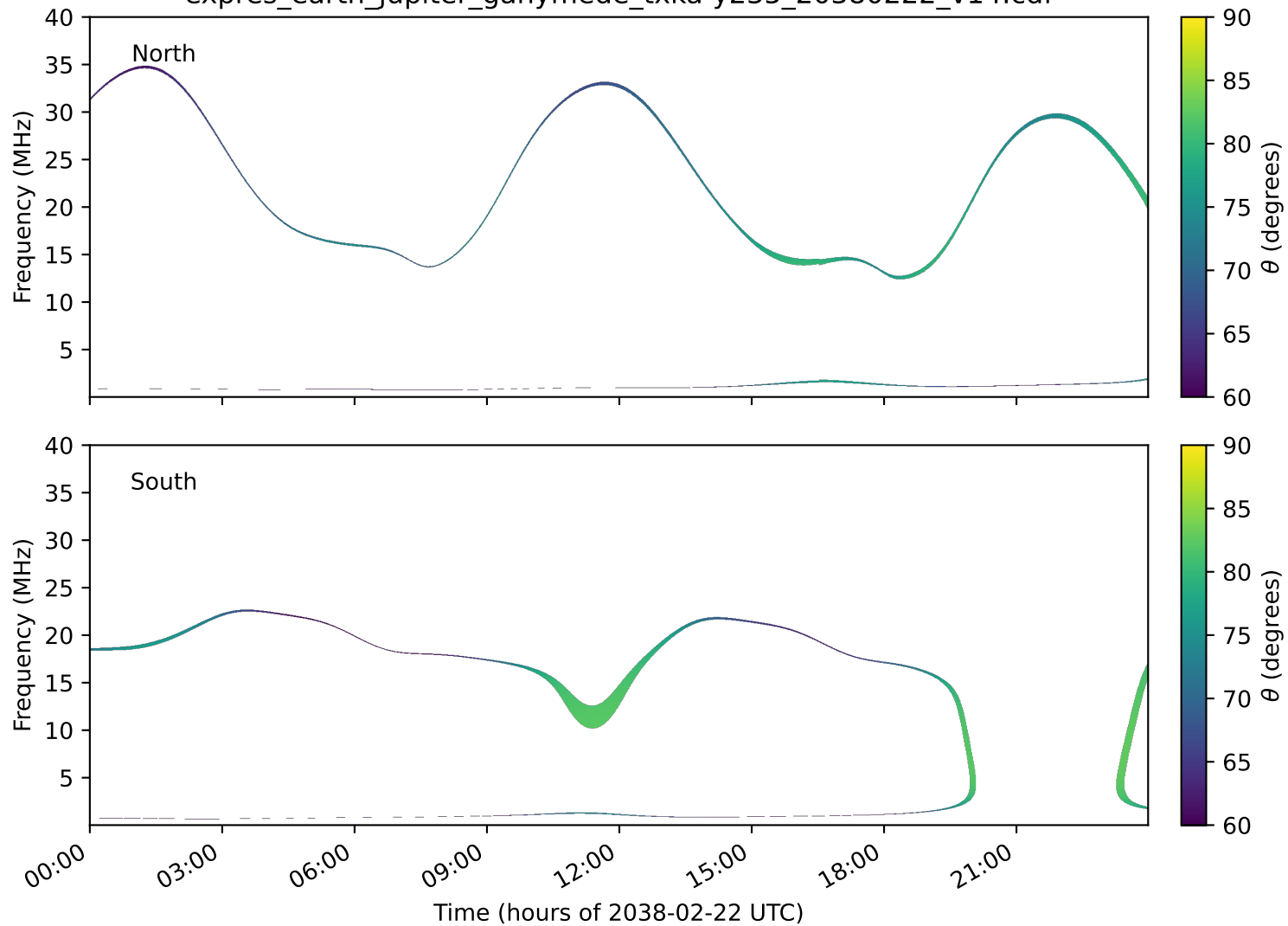
expres_earth_jupiter_ganymede_txka-y235_20380222_v14.cdf
