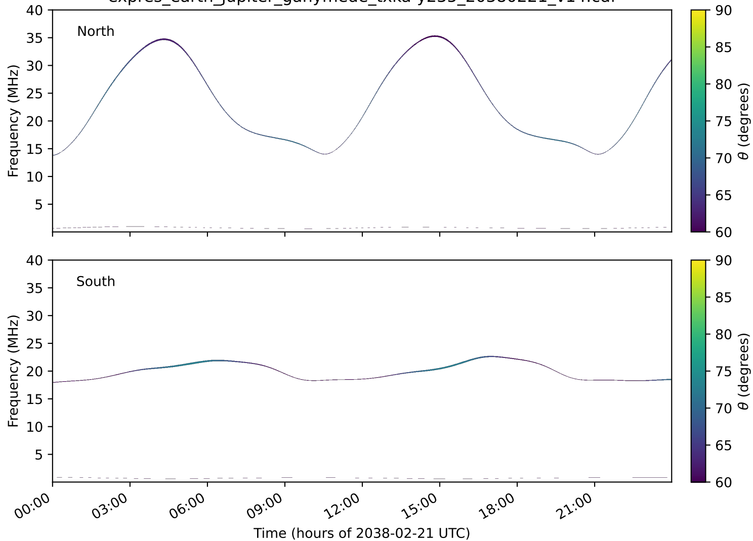
expres_earth_jupiter_ganymede_txka-y235_20380221_v14.cdf
