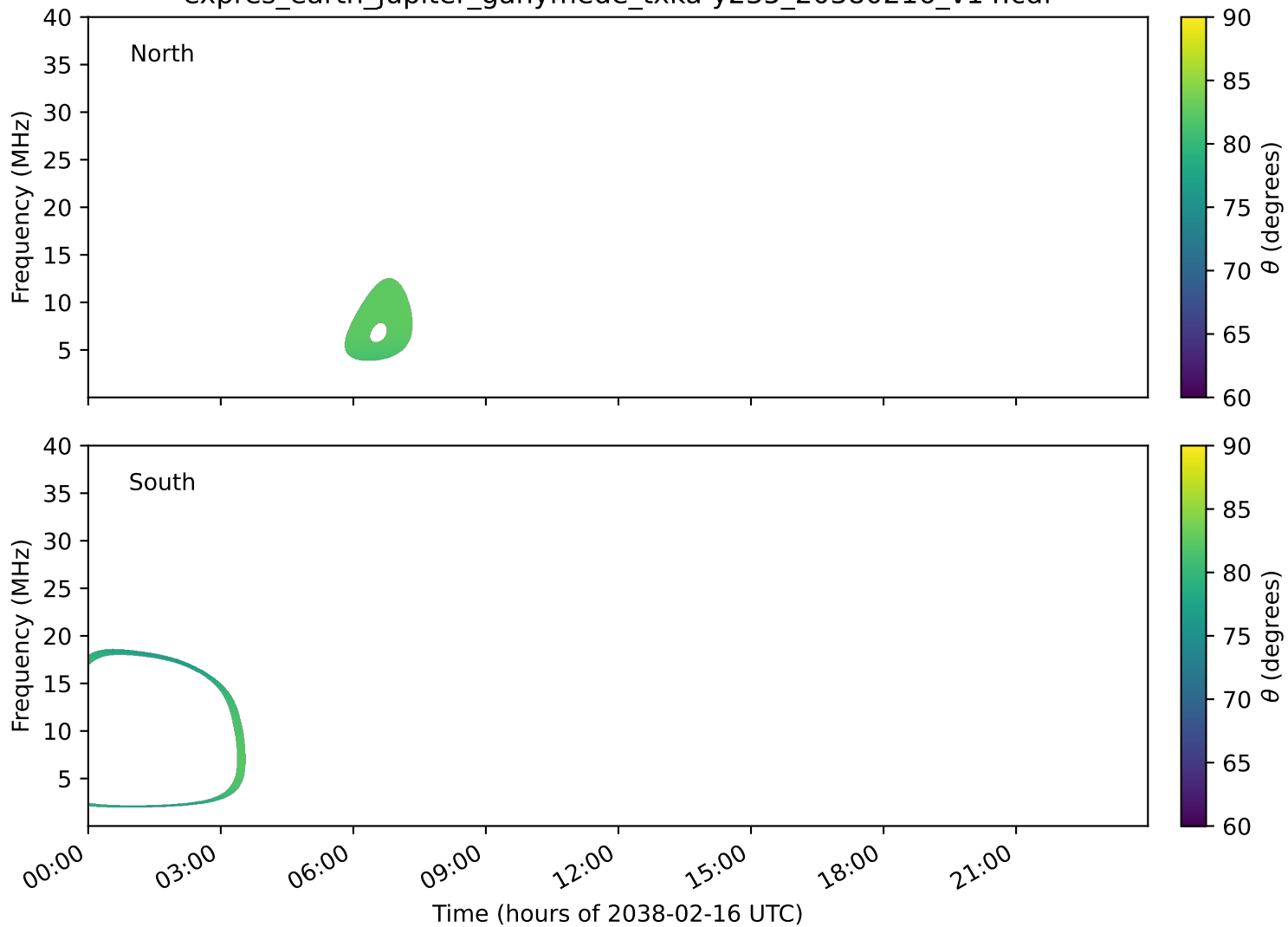
expres_earth_jupiter_ganymede_txka-y235_20380216_v14.cdf
