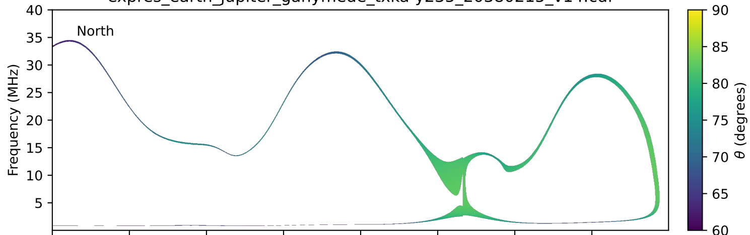
expres_earth_jupiter_ganymede_txka-y235_20380215_v14.cdf
