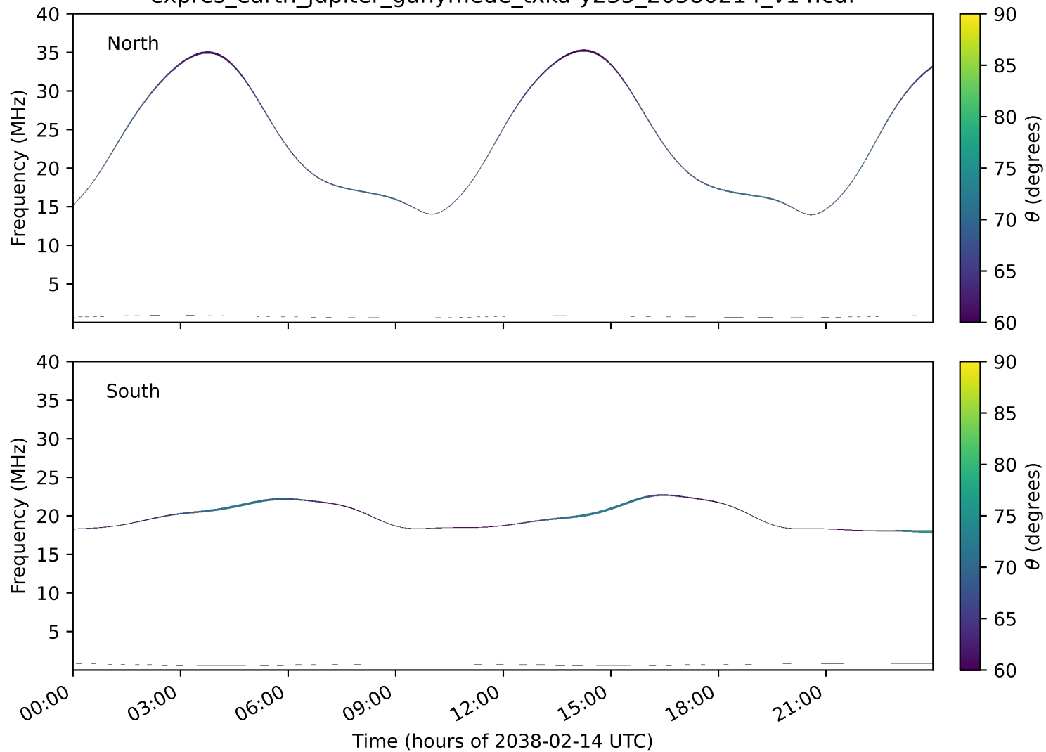
expres_earth_jupiter_ganymede_txka-y235_20380214_v14.cdf
