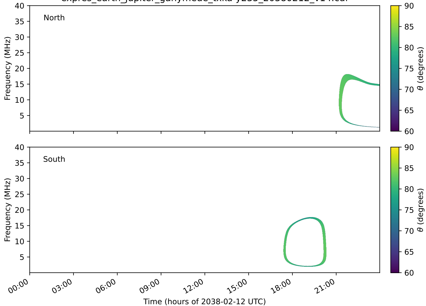
expres_earth_jupiter_ganymede_txka-y235_20380212_v14.cdf
