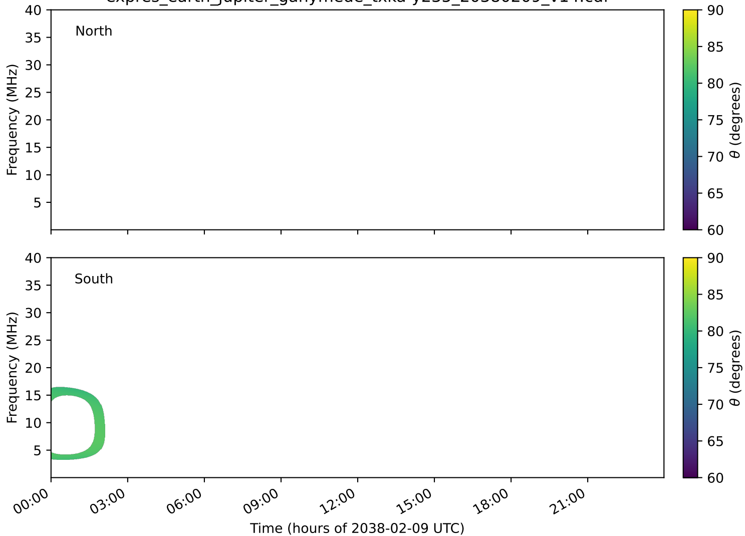
expres_earth_jupiter_ganymede_txka-y235_20380209_v14.cdf
