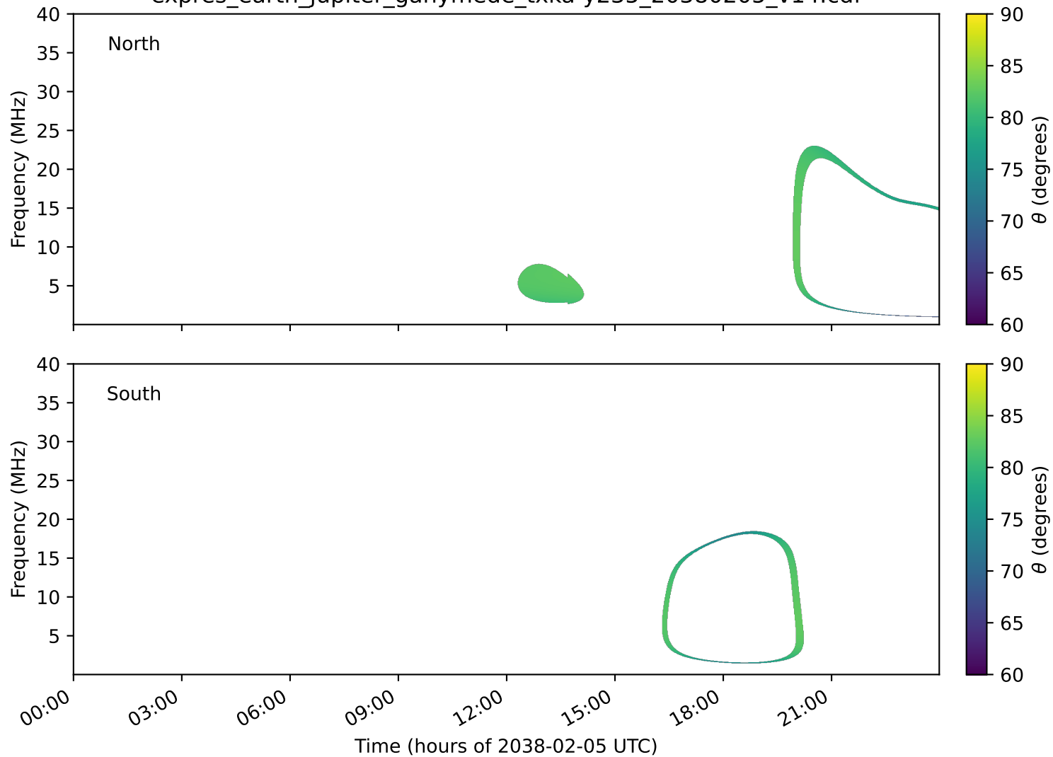
expres_earth_jupiter_ganymede_txka-y235_20380205_v14.cdf
