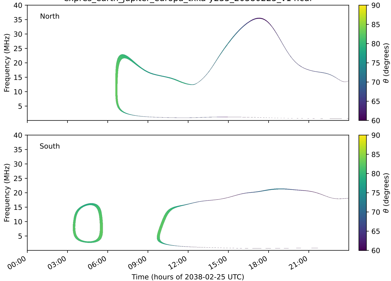
expres_earth_jupiter_europa_txka-y235_20380225_v14.cdf
