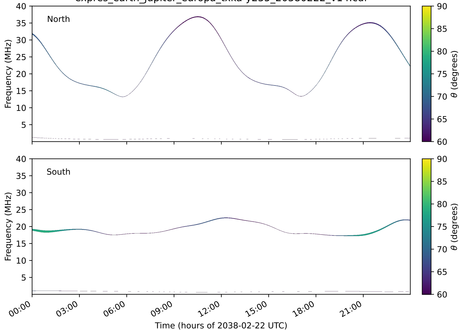
expres_earth_jupiter_europa_txka-y235_20380222_v14.cdf
