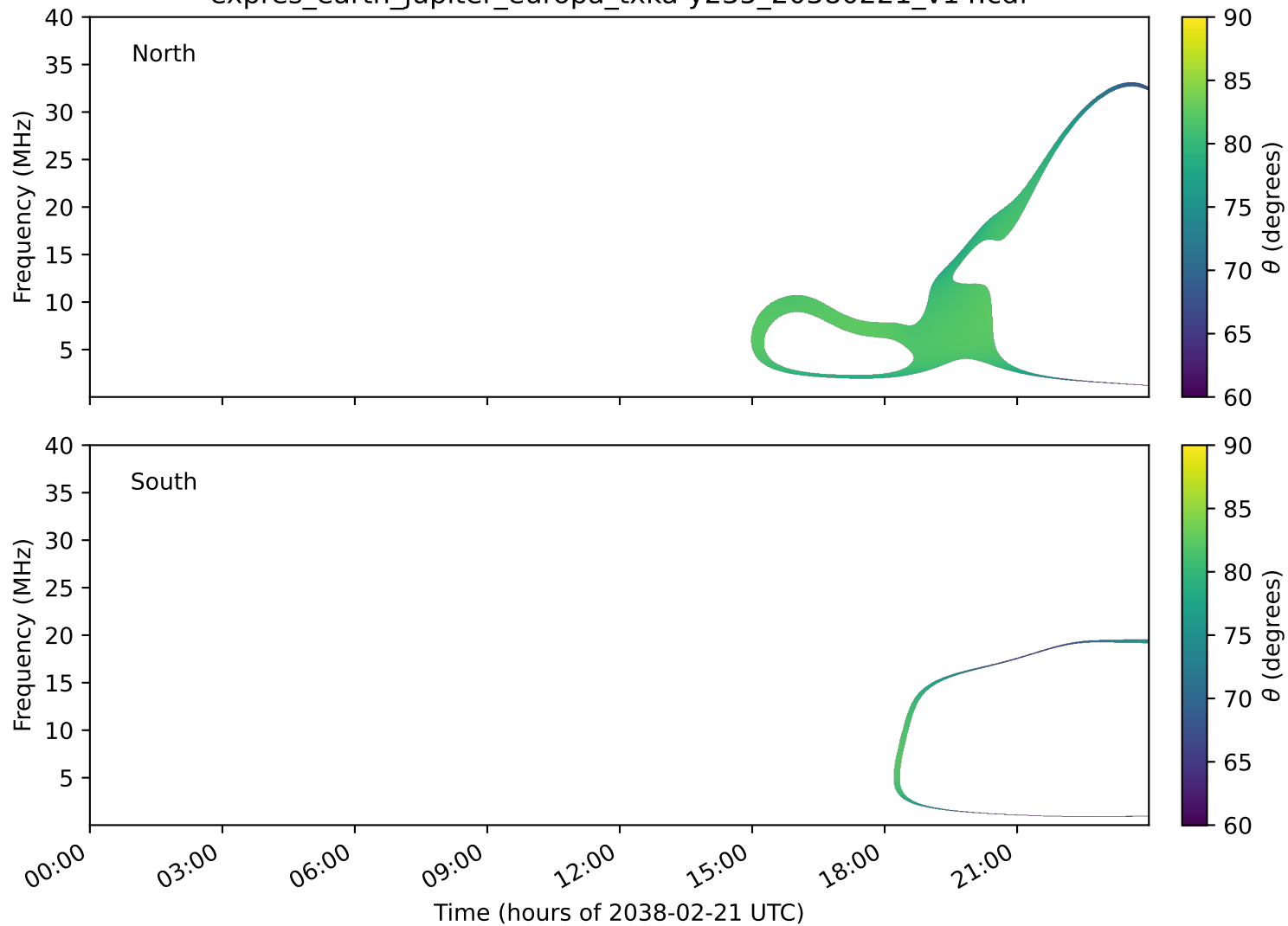
expres_earth_jupiter_europa_txka-y235_20380221_v14.cdf
