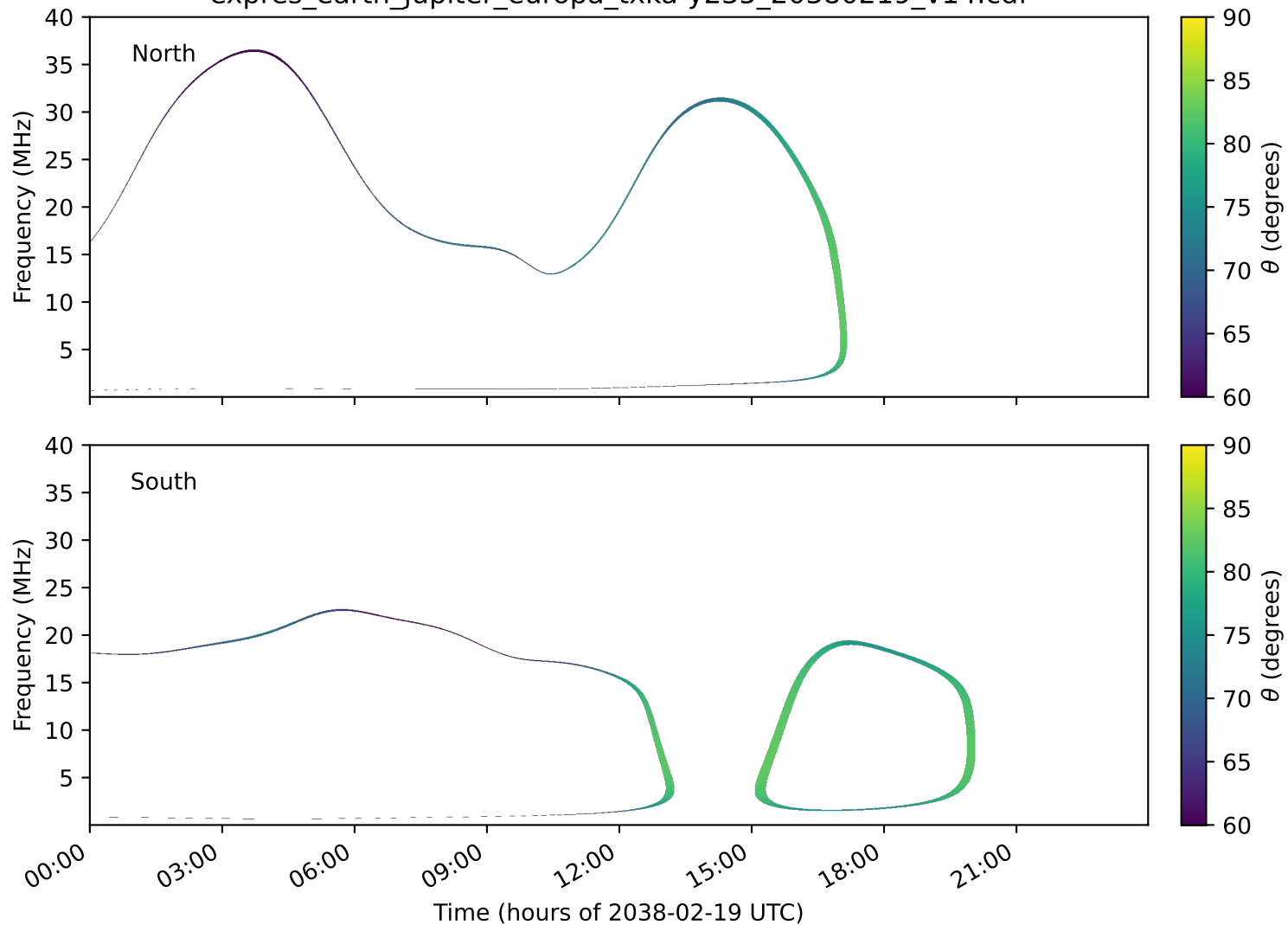
expres_earth_jupiter_europa_txka-y235_20380219_v14.cdf
