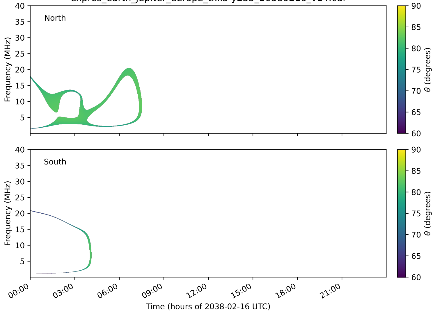
expres_earth_jupiter_europa_txka-y235_20380216_v14.cdf
