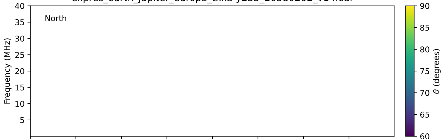
expres_earth_jupiter_europa_txka-y235_20380202_v14.cdf
