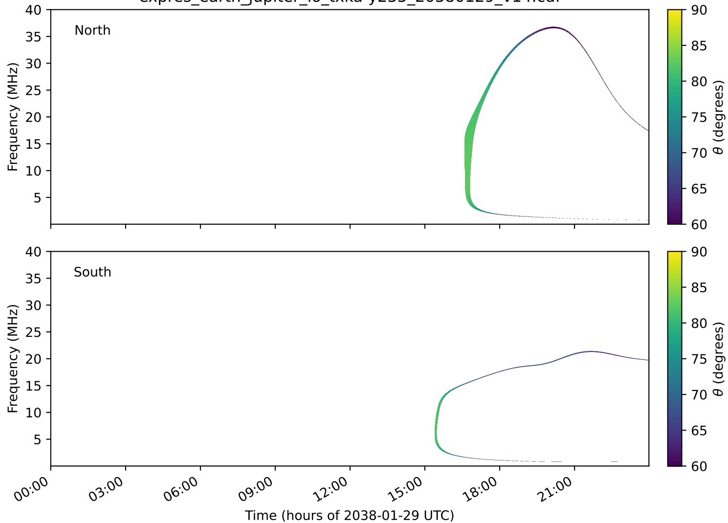
expres_earth_jupiter_io_txka-y235_20380129_v14.cdf
