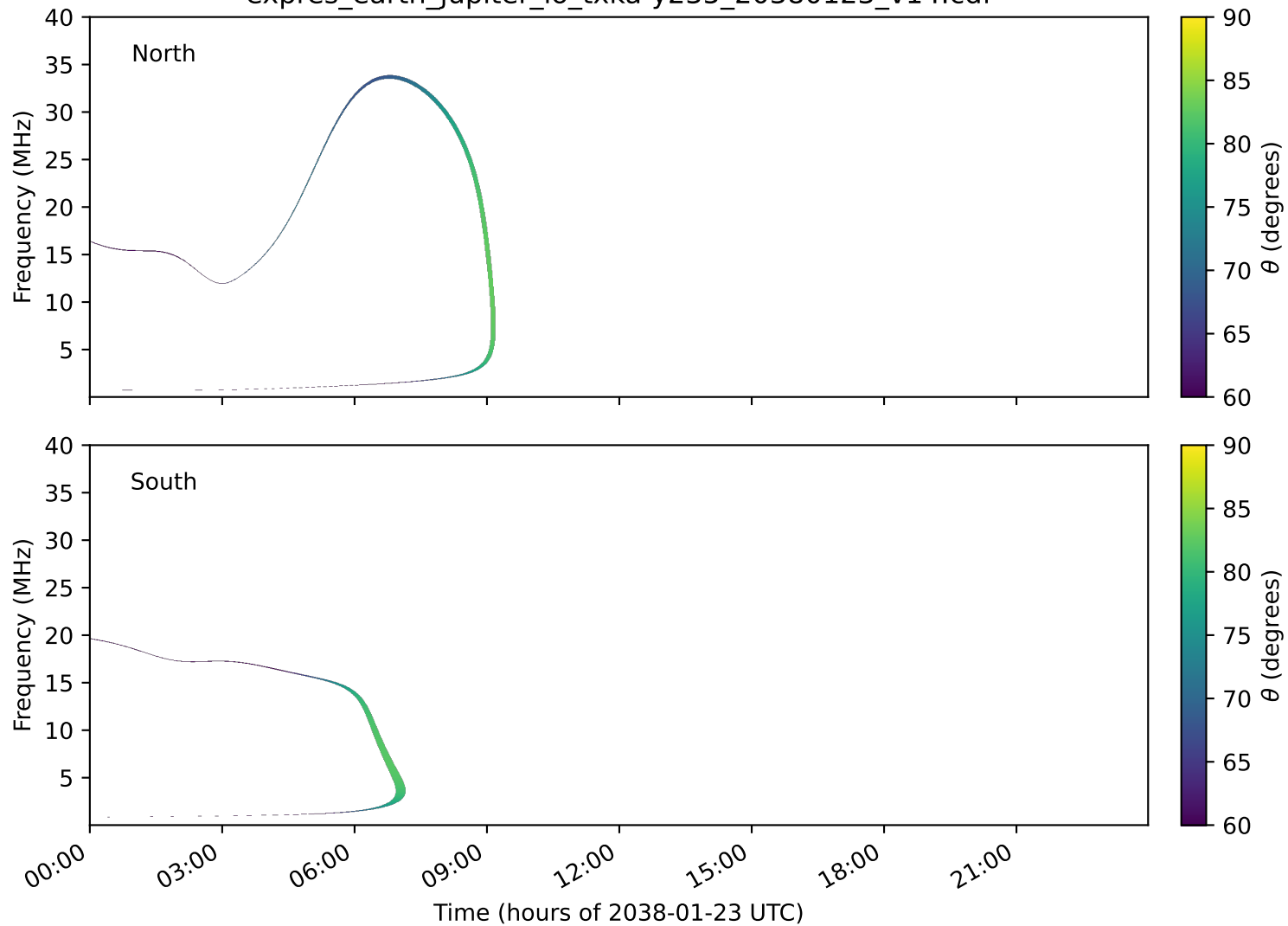
expres_earth_jupiter_io_txka-y235_20380123_v14.cdf
